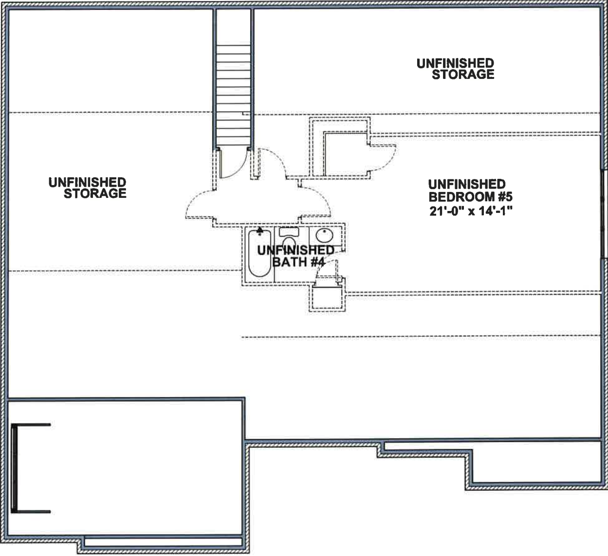
OPTIONAL ATTIC PLAN
